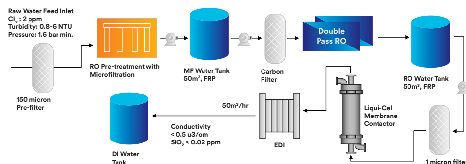
Figure 1. Schematic Diagram of Water Treatment System (RO-LMC-EDI)
