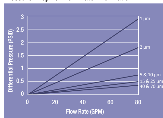
Graph 1: 3M™ 740 Series Filter Cartridges Pressure Drop vs. Flow Rate Information
