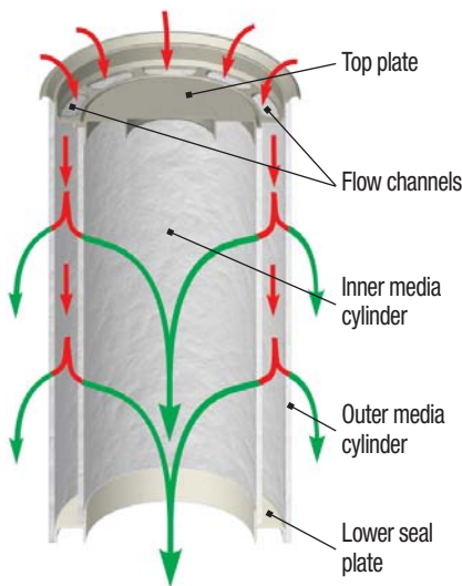
Figure 1: 3M™ DF Series flow path
