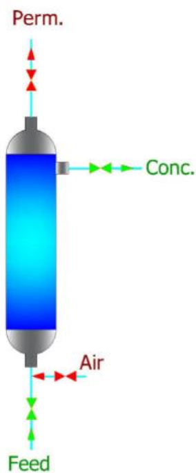
1.1 Forward Flush
