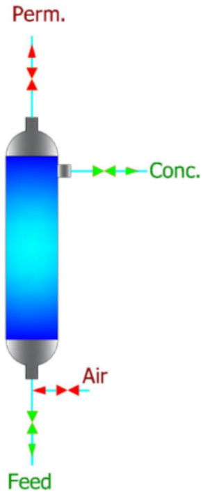
2.1 Drain
