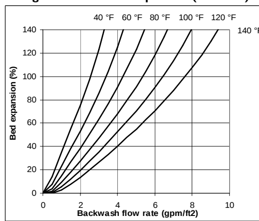
Figure 4 Backwash Expansion (US units)
