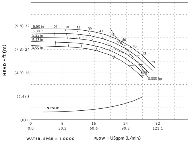
2 × 1.5 × 5.5 - 1800 RPM
