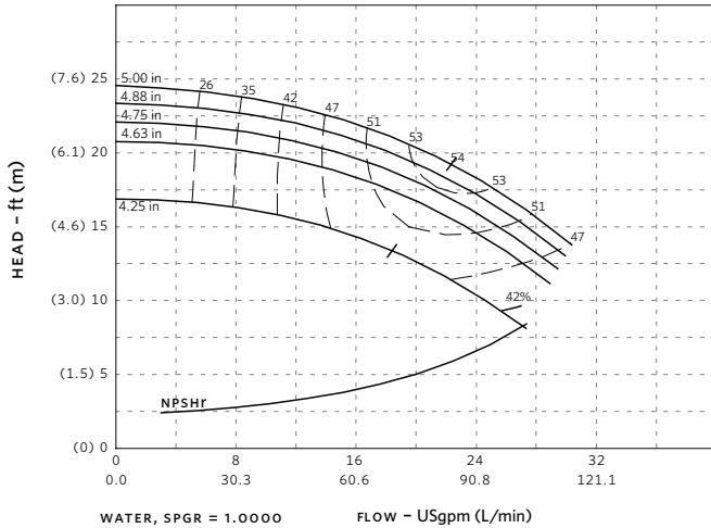
1.5 × 1.25 × 5.5 - 1800 RPM
