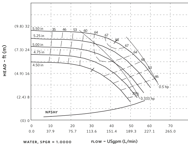
2 × 1.5 × 5.5 - 1800 RPM
