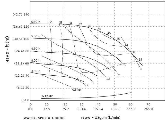
2 × 1.5 × 5.5 - 3600 RPM
