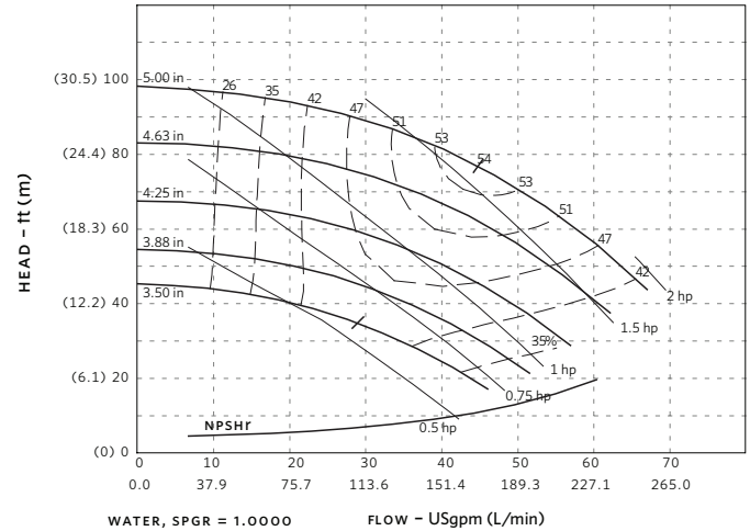
1.5 × 1.25 × 5.5 - 3600 RPM
