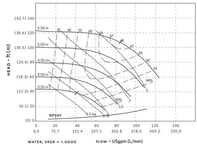
2 × 1.5 × 5.5 - 3600 RPM
