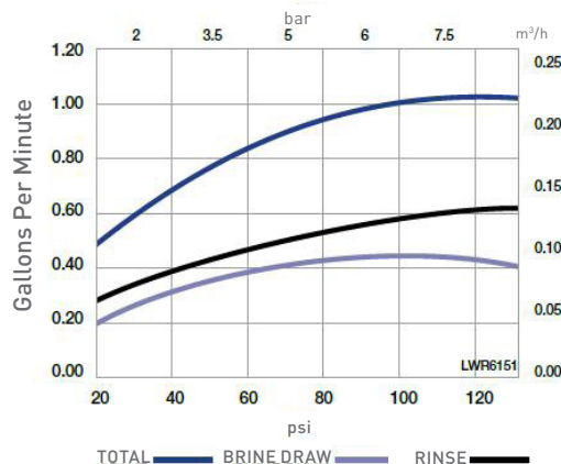
Injector «L» (Orange) For 13- and 14-inch Tanks
