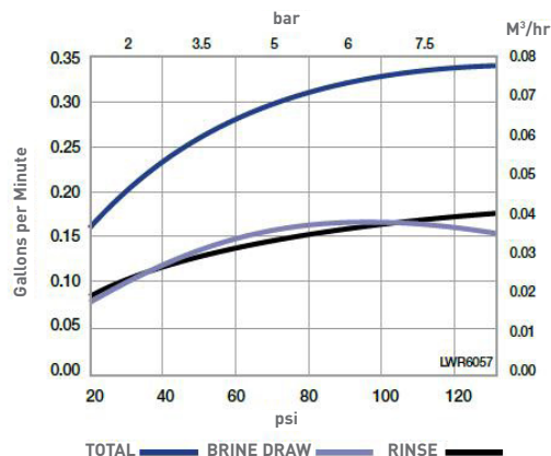
Injector "F"(Peach) For 7-inch Tanks
