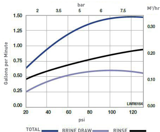
Injector "L"(Orange) For 13-inch and 14-inch Tanks
