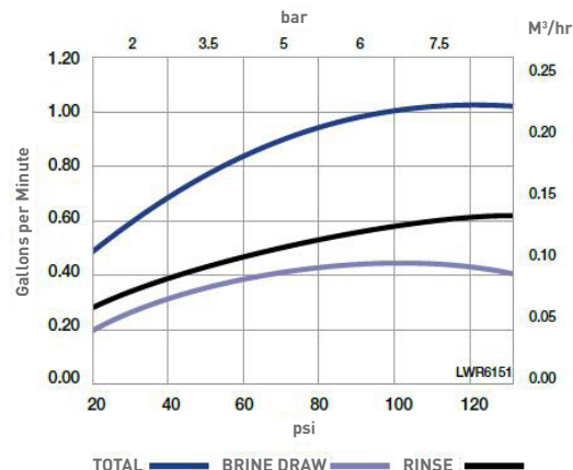
Injector "K"(Pink) For 12-inch Tanks
