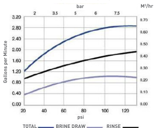
Injector "Q"(Purple) For 18-inch Tanks
