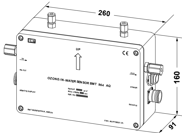
dimensional outline
