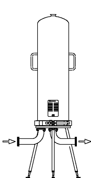
1 to 8 fold cartridge housing (Design with quick closure)
