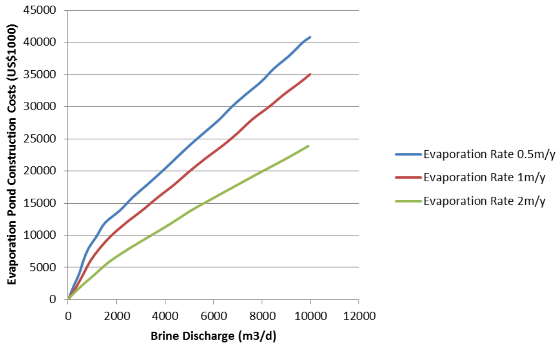
Figure 1, Construction cost for an evaporation brine disposal pond system
