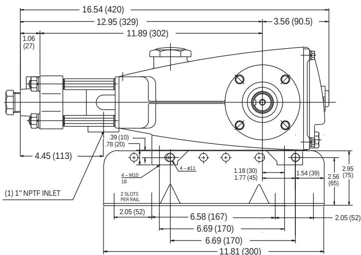
Models 623, 621, 625, 820, 821, 825, 1010, 1011, 1015
