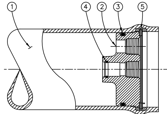
SECTION THROUGH END CLOSURE
