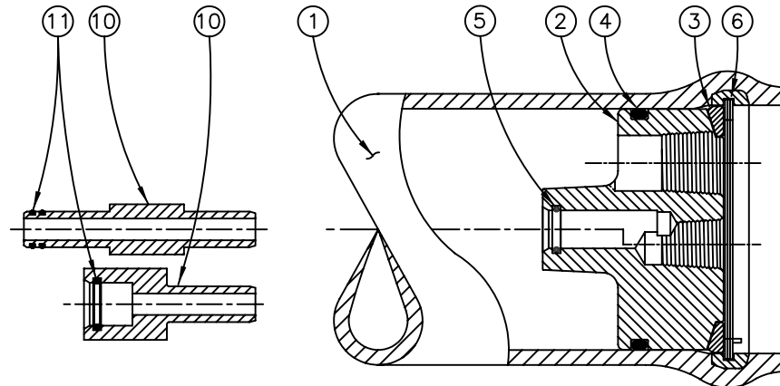
SECTION THROUGH END CLOSURE
