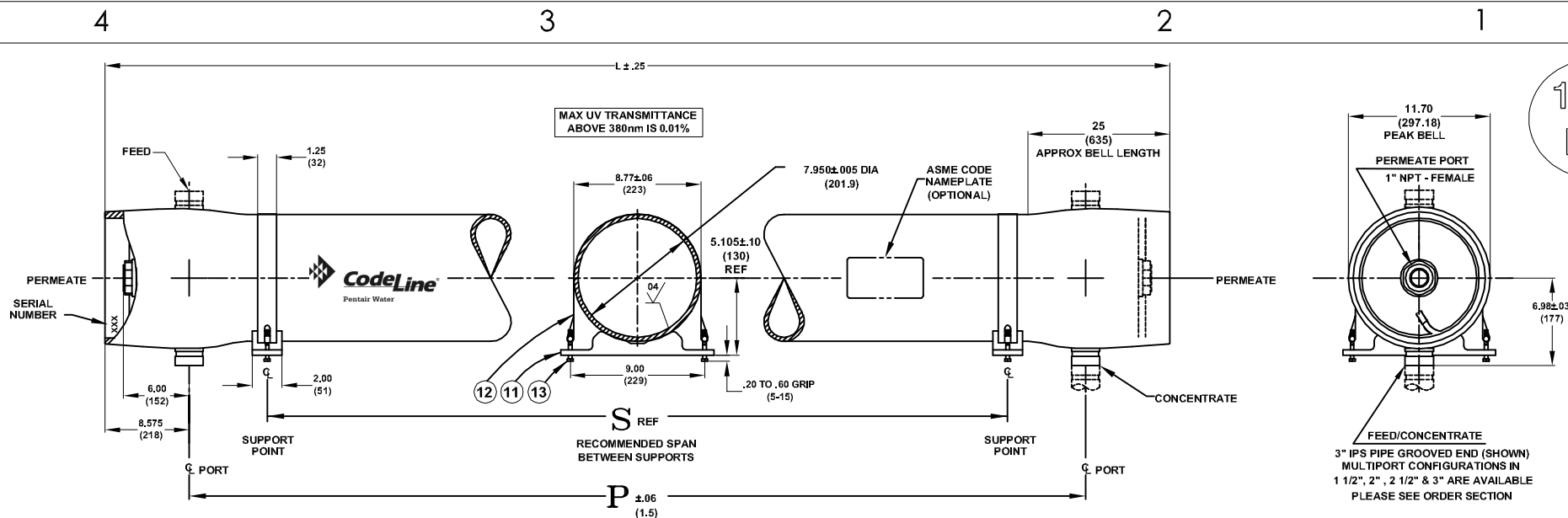
VIEW AT CENTER SUPPORT CENTER VESSEL ON 2 OR 3 SUPPORTS AT SPAN(S) "S" : 3 SUPPORTS REQUIRED FOR LENGTHS -4 AND ABOVE
