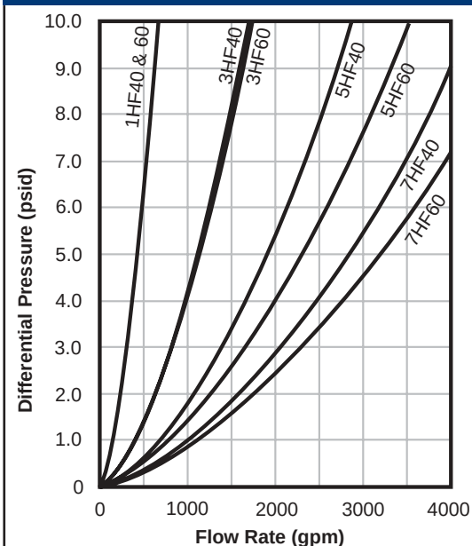
Figure 4 – Typical Housing Flow Rates
