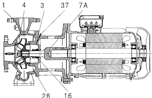
VERSION WITH MOTOR UP TO 7,5 KW COMPRESSED
