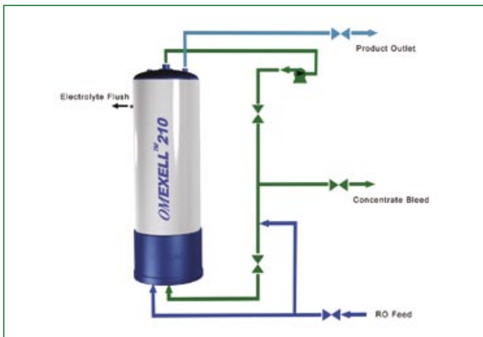
Figure 3: Flow Loop
