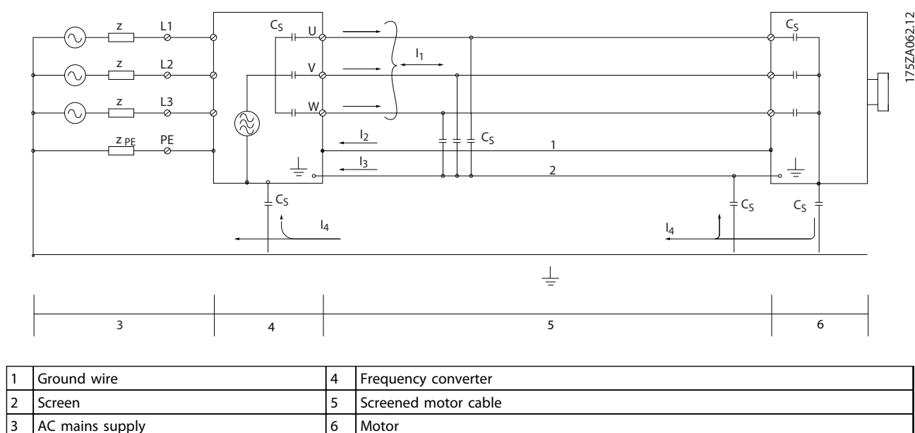
Illustration 5.3 Situation that Generates Leakage Currents
