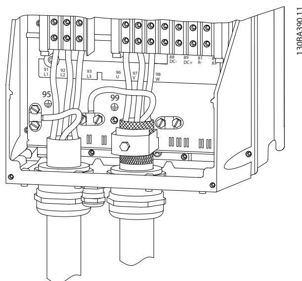
Illustration 9.35 Motor Connection Enclosures C1 and C2 (IP21/NEMA Type 1 and IP55/66/NEMA Type 12)
