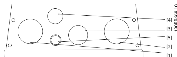
Illustration 9.10 B2 - IP21
