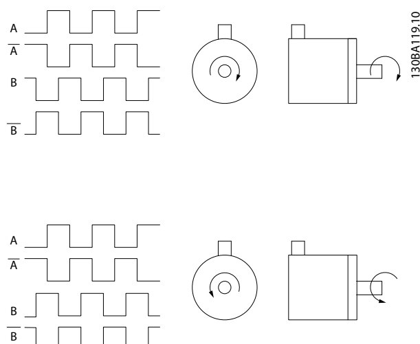
Illustration 11.5 Rotation Direction
