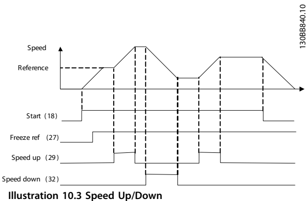
Illustration 10.3 Speed Up/Down
