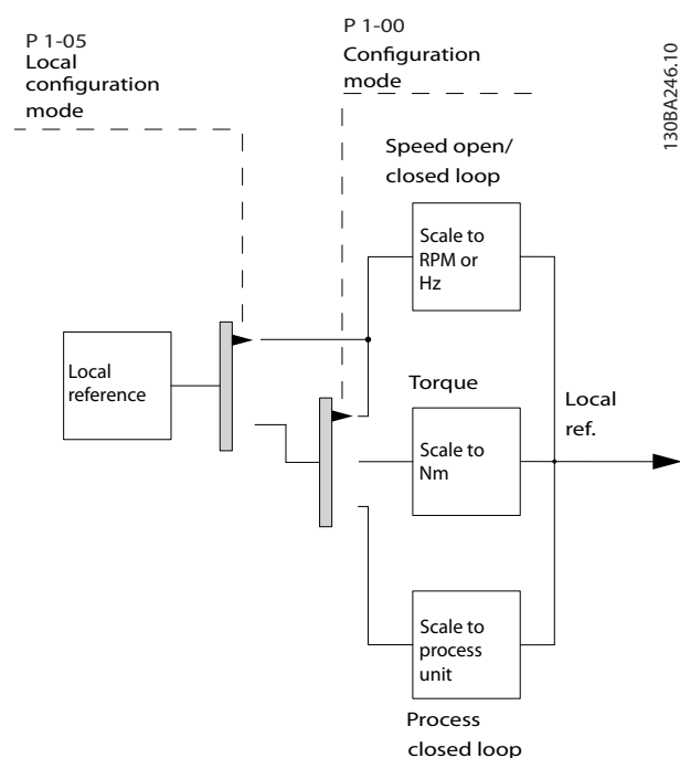
Illustration 3.12 Configuration Mode
