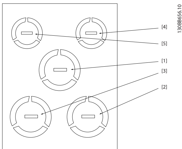
Illustration 9.2 A3 - IP21
