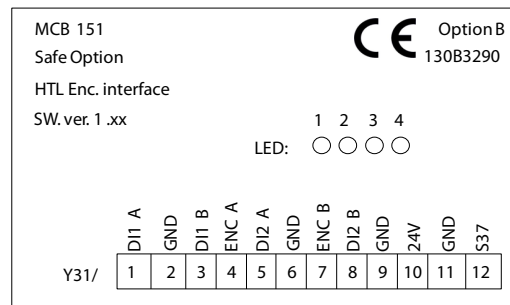
Illustration 11.21 MCB 151
