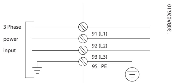
Illustration 9.16 Mains Connection
