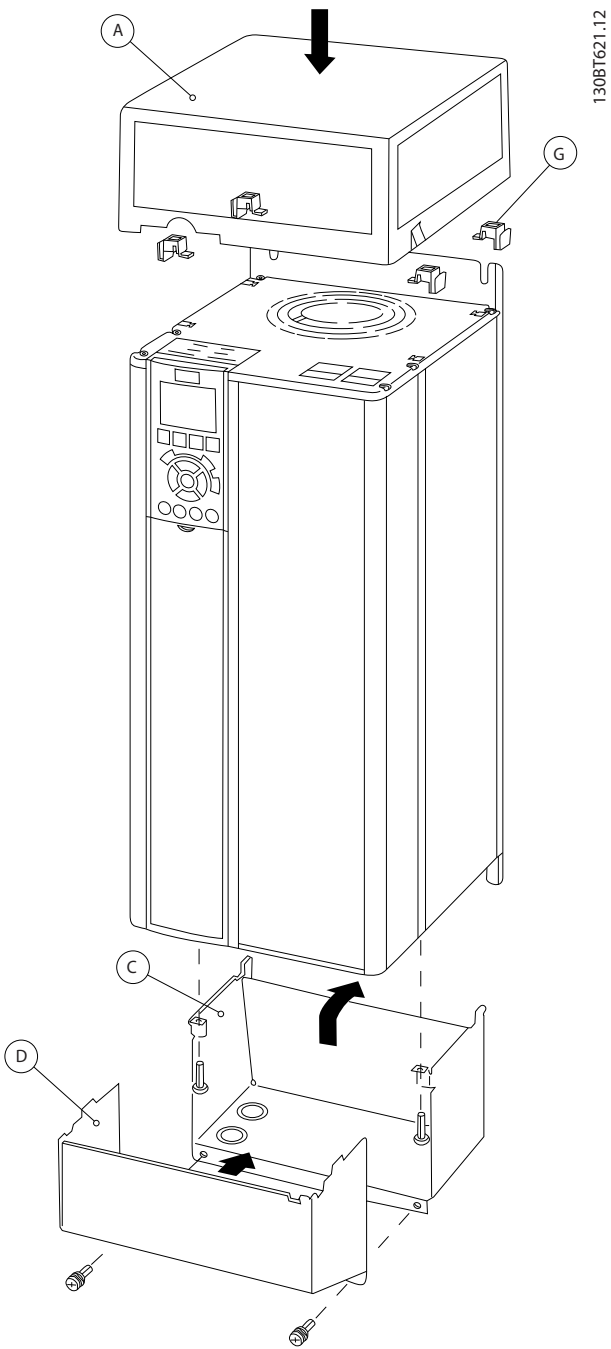
Illustration 11.26 Enclosure Types B4 - C3 - C4
