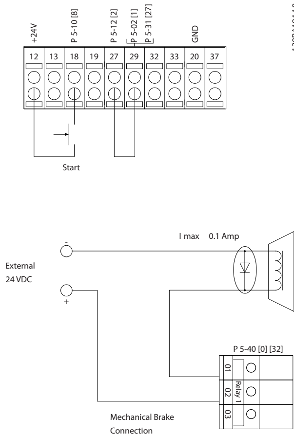
Illustration 10.6 External Electro-mechanical Brake
