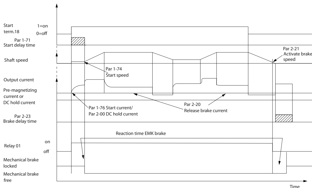
Illustration 4.2 Mechanical Brake
