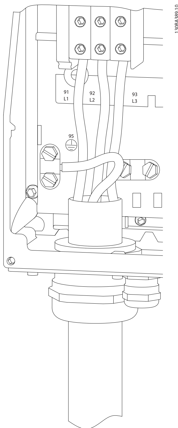
Illustration 9.26 Mains Connection Enclosures C1 and C2 (IP21/NEMA Type 1 and IP55/66/NEMA Type 12).
