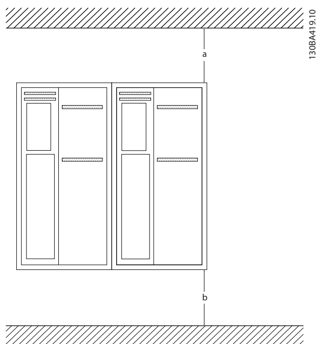
Illustration 8.2 Clearance
