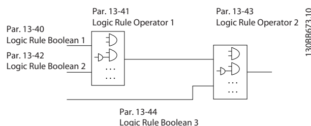
Illustration 4.7 Logic Rules
