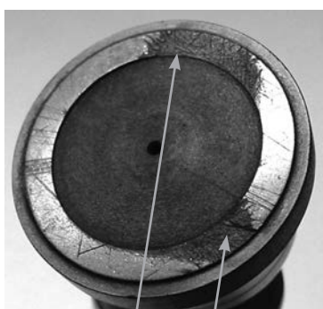
Abrasive wear of the piston shoes. All pistons must be replaced immediately.
