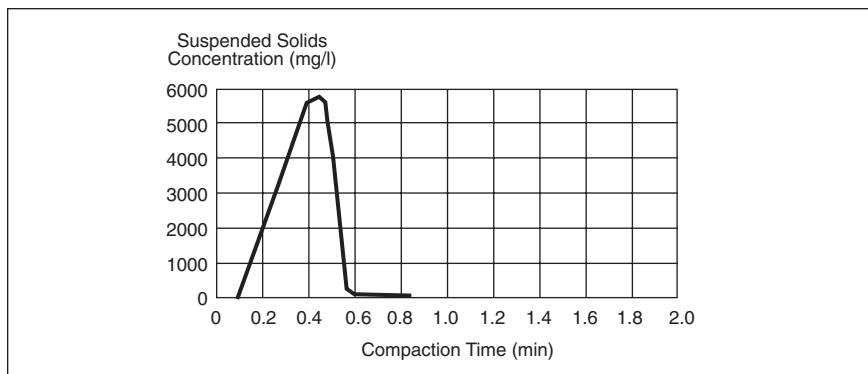
Figure 8. Compaction Effluent Profile Suspended Solids vs. Backwash Time
