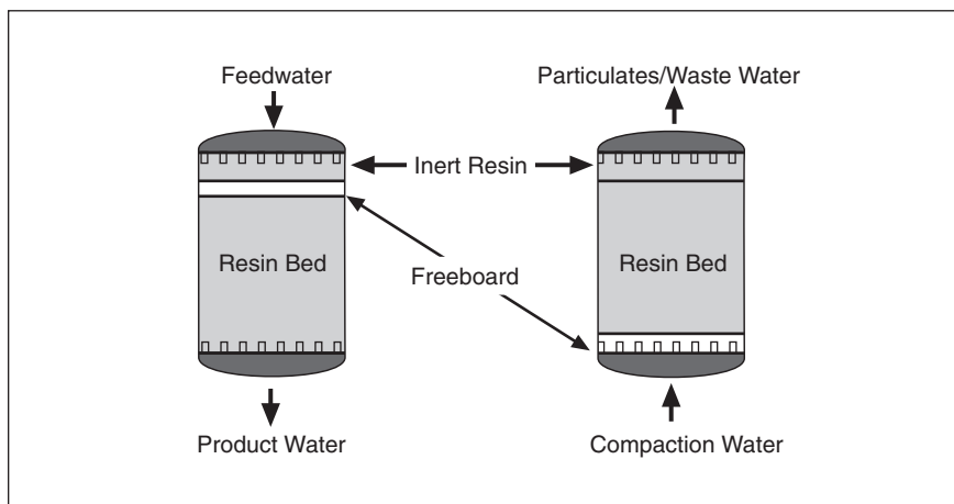
Figure 5. UPCORE System - Compaction
