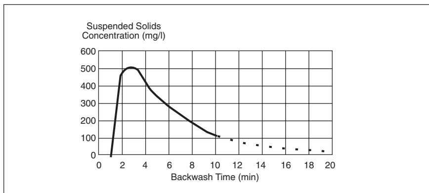
Figure 7. Backwash Effluent Profile Suspended Solids vs. Backwash Time
