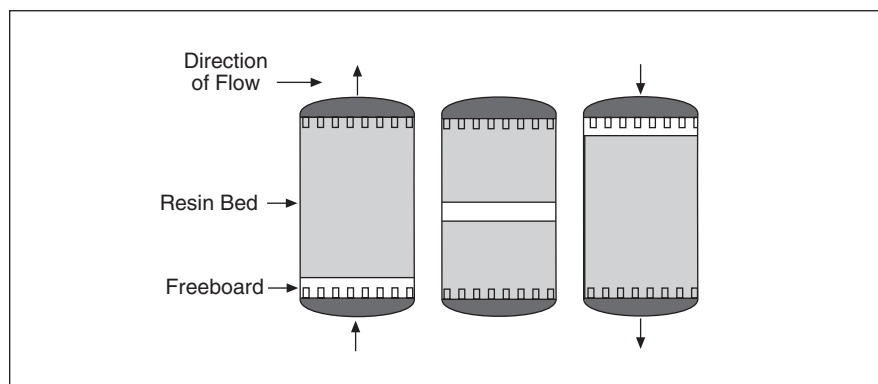
Figure 3. Movement of Freeboard from Bottom to Top
