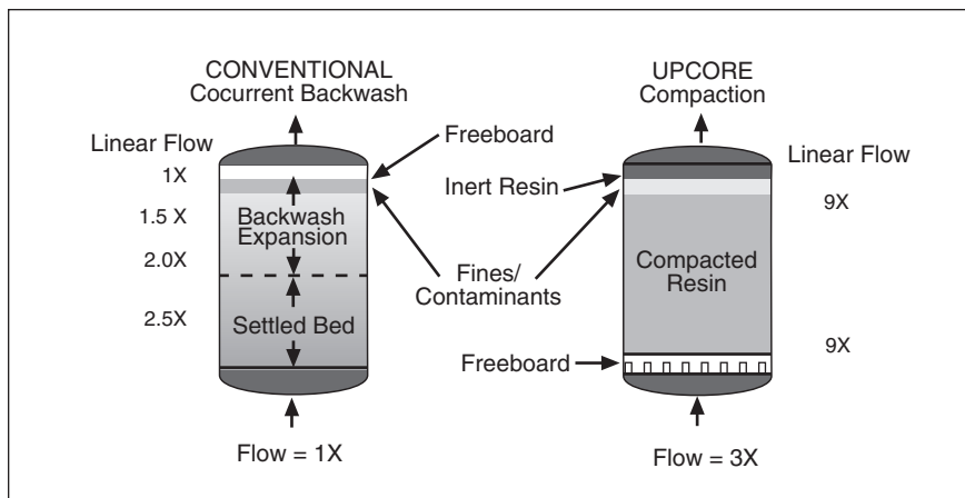
Figure 6. Solids Removal Mechanisms
