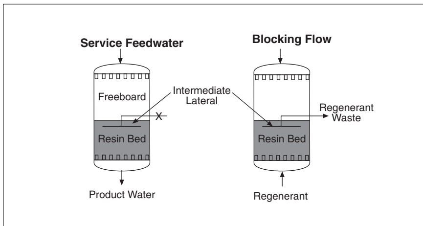
Figure 2. Blocking Flow Countercurrent Systems
