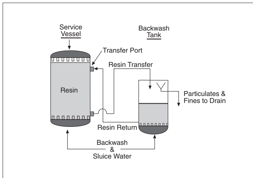
Figure 4. Fluidized Bed Backwash System
