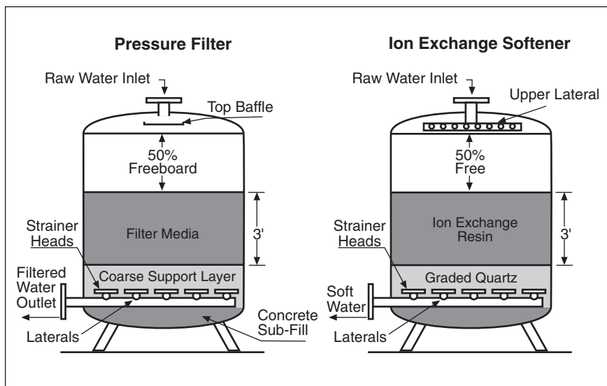
Figure 1. Design Comparisons. Pressure Filters and Ion Exchange Softeners
