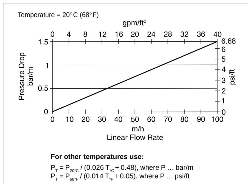
Figure 2. Pressure drop
