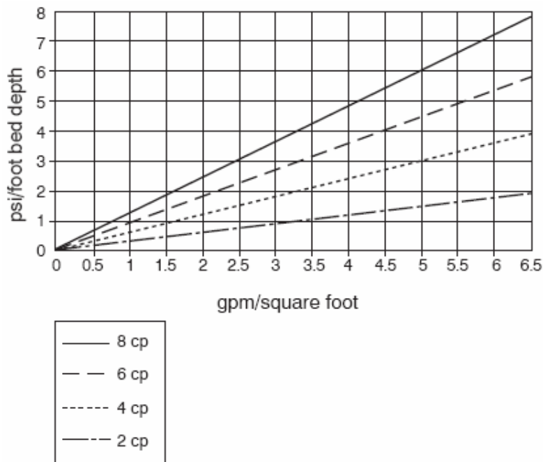
Figure 1. Pressure Drop
