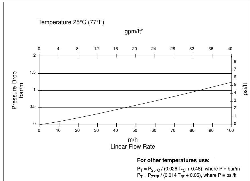
Figure 2. Pressure drop
