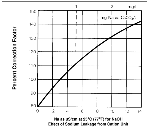
Figure 6. Sodium leakage correction for co-current operation
