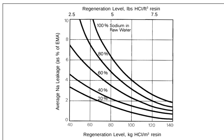
Figure 6. Average Na leakage from DOWEX HCR-S resin in co-current operation with HCl as regenerant
