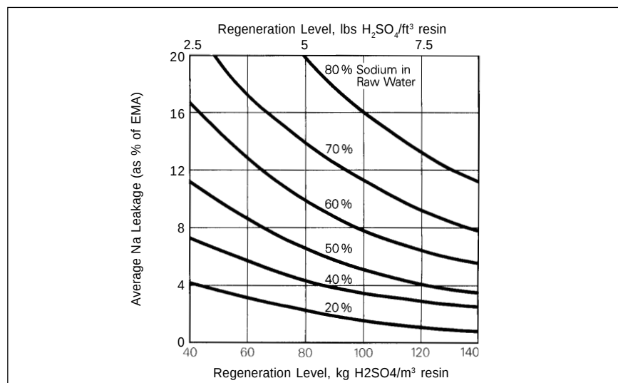
Figure 7. Average Na leakage from DOWEX HCR-S resin in co-current operation with \text{H}_2\text{SO}_4 as regenerant
