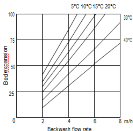
Figure 1: Backwash Expansion
