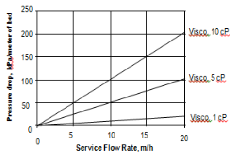
Figure 2: Pressure Drop
