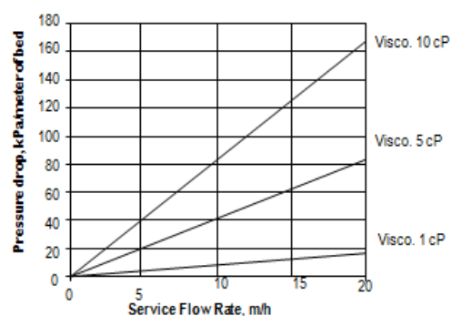
Figure 2: Pressure Drop
