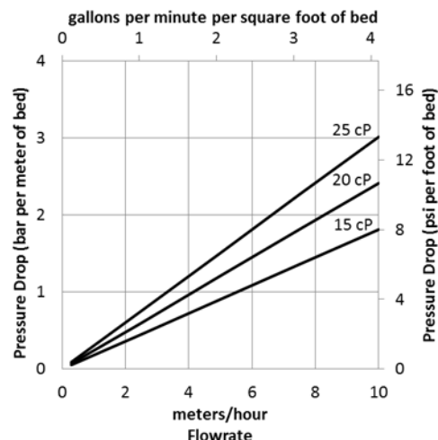
Figure 2: Pressure Drop
