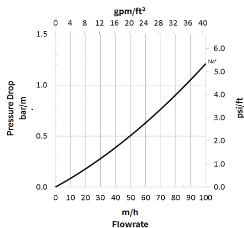
Figure 2: Pressure Drop
