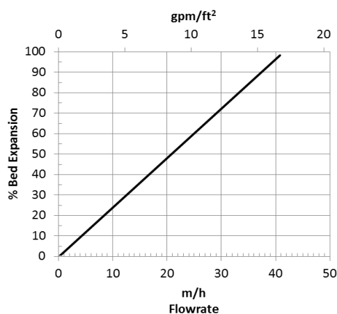
Figure 1: Backwash Expansion Temperature = 25°C (77°F)
