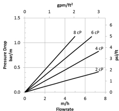
Figure 2: Pressure Drop Viscosity = 2 – 8 cP
