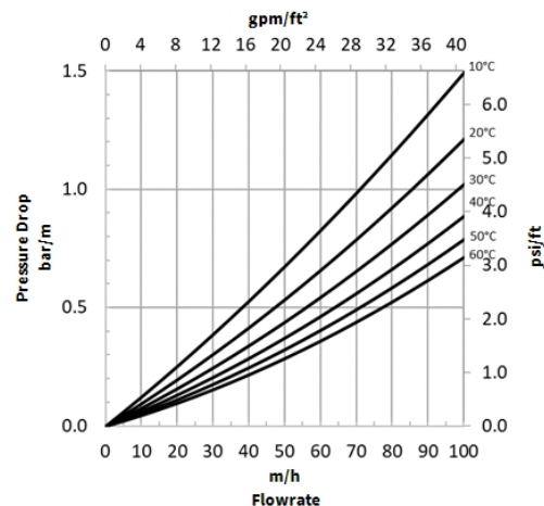
Figure 2: Pressure Drop
