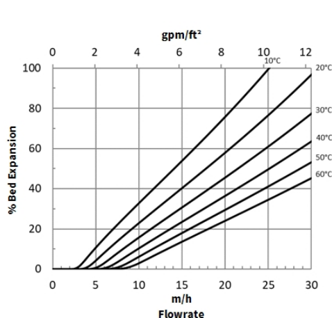
Figure 1: Backwash Expansion
