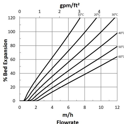
Figure 1: Backwash Expansion
