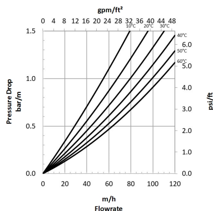
Figure 2: Pressure Drop
