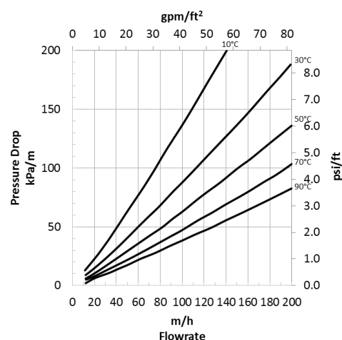
Figure 2: Pressure Drop
