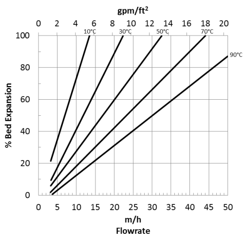
Figure 1: Backwash Expansion
