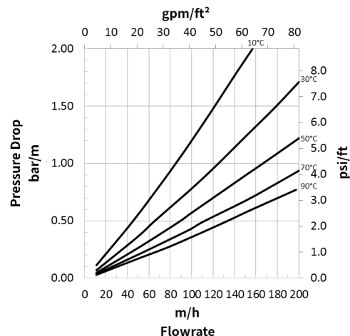
Figure 2: Pressure Drop
