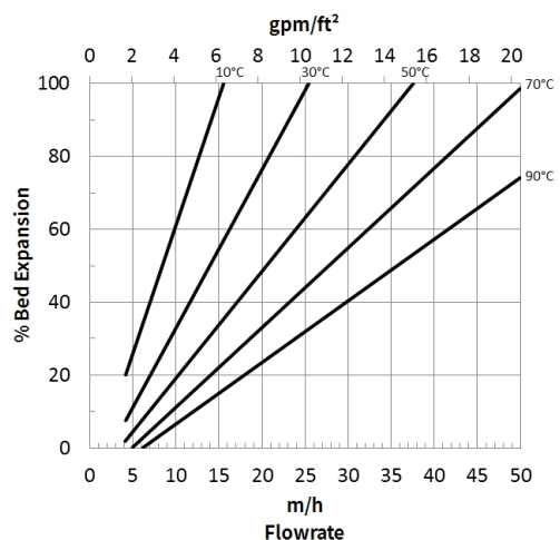
Figure 1: Backwash Expansion
