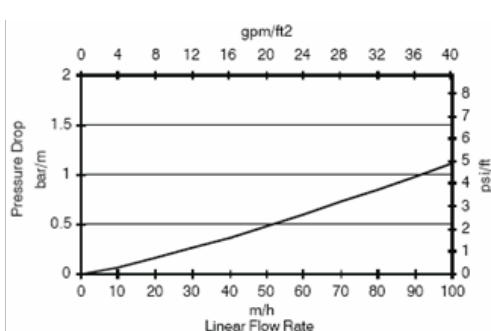
Figure 2: Pressure Drop
