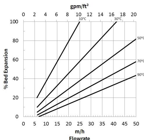
Figure 1: Backwash Expansion
