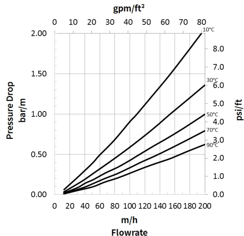
Figure 2: Pressure Drop
