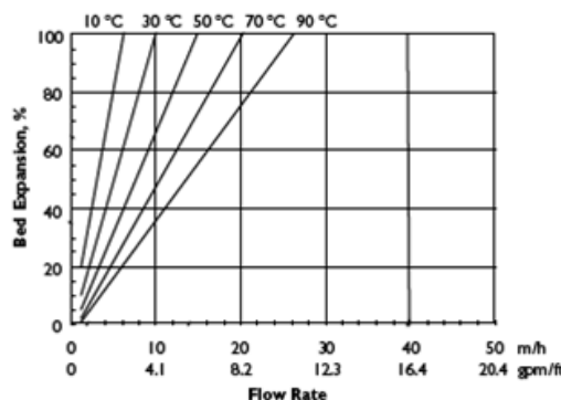
Figure 1: Backwash Expansion
