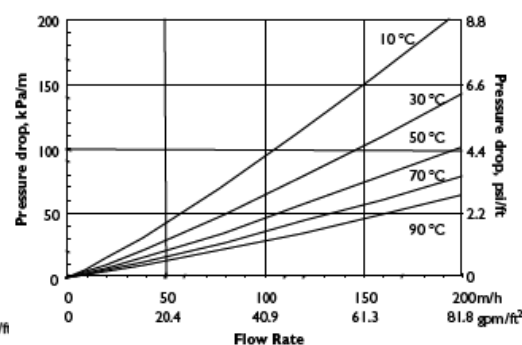
Figure 2: Pressure Drop
