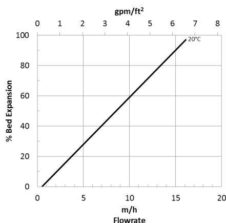
Figure 1: Backwash Expansion
