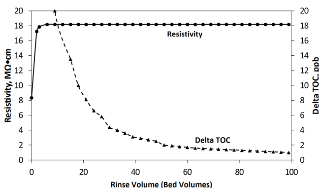
Figure 2: Resistivity and TOC Rinse Performance
