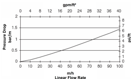
Figure 1: Pressure Drop
