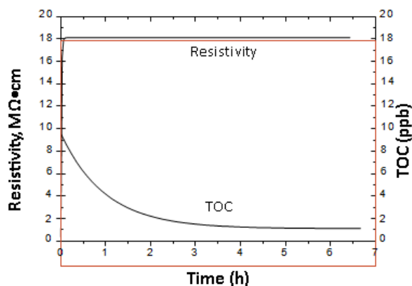
Figure 3: Resistivity and TOC Rinse Performance
