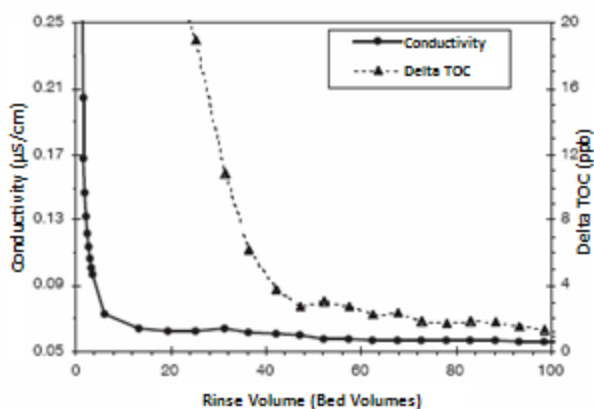
Figure 3: Conductivity and TOC Rinse-down
