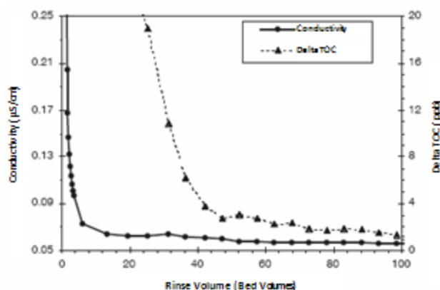
Figure 3: Conductivity and TOC Rinse-down
