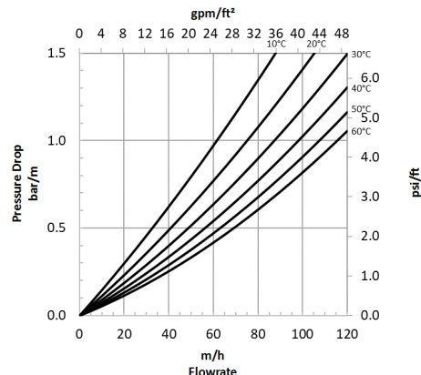
Figure 2: Pressure Drop
