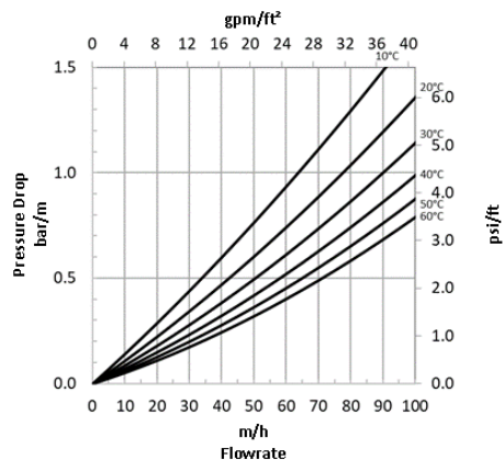
Figure 1: Pressure Drop
