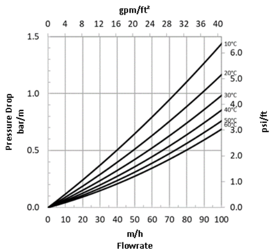
Figure 1: Pressure Drop
