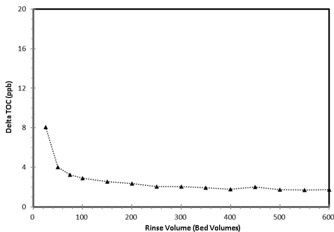
Figure 2: TOC Rinse-down
