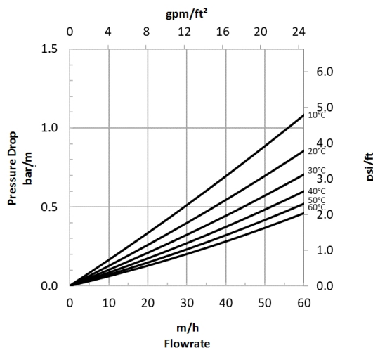
Figure 1: Pressure Drop
