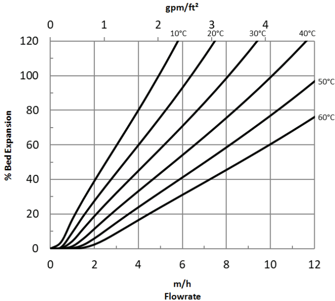
Figure 1: Backwash Expansion
