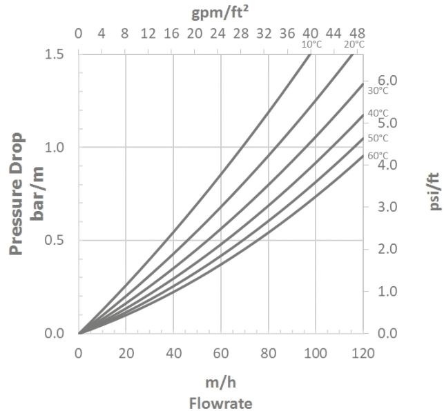
Figure 2: Pressure Drop
