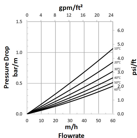
Figure 2: Pressure Drop
